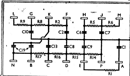
Sketch showing the connecting panel and internal circuit of the large component assembly indicated in the under-chassis view, where an arrow shows the direction in which it is viewed.
